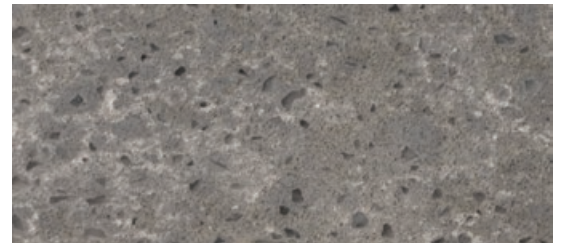
3018 Full Moon
